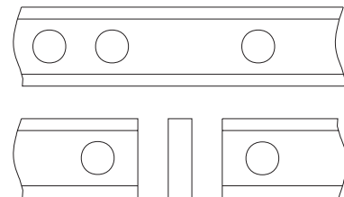
Processing: Ø8 hole for additional fastening mechanisms; cutting and double Ø8 hole
