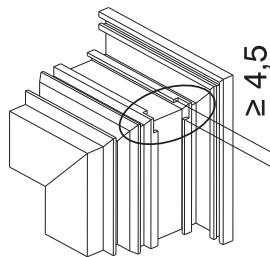
Tabs removal
