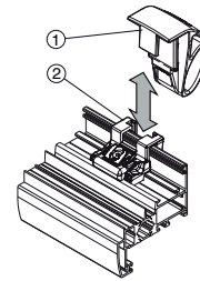
Lever Away (1) and support (2)
