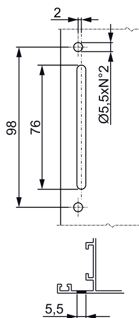
C/C distance machining 98 mm
