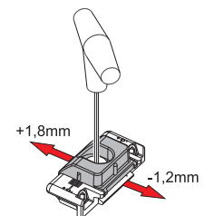
Compression adjustment
