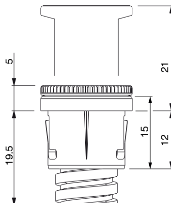
Dimensions Art. 06501
