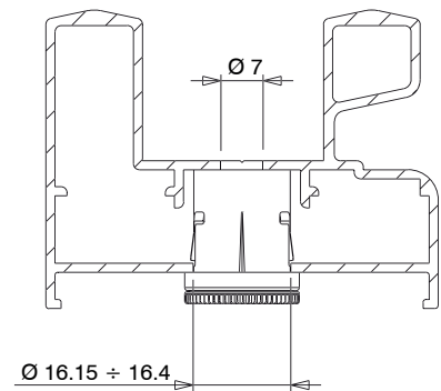
Machining Art. 06502
