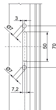
C/C distance machining 70 mm
