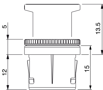
Dimensions Art. 06500
