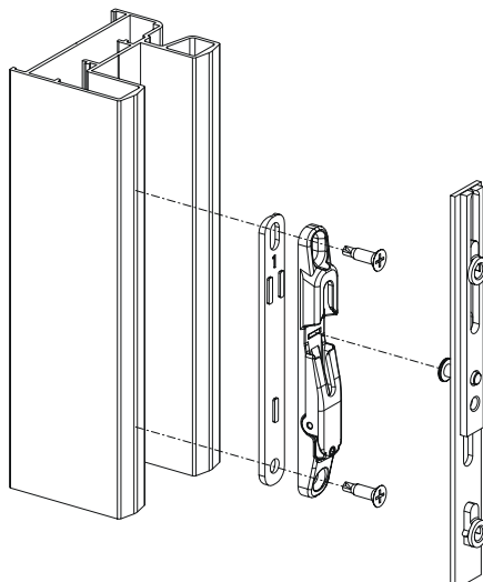
Micro-ventilation counterplate
