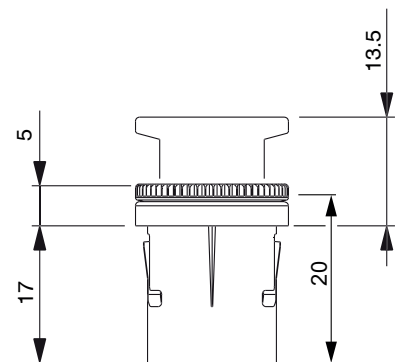
Dimensions Art. 06502
