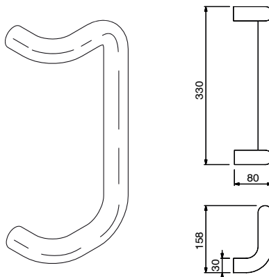
Double curved brass handle
