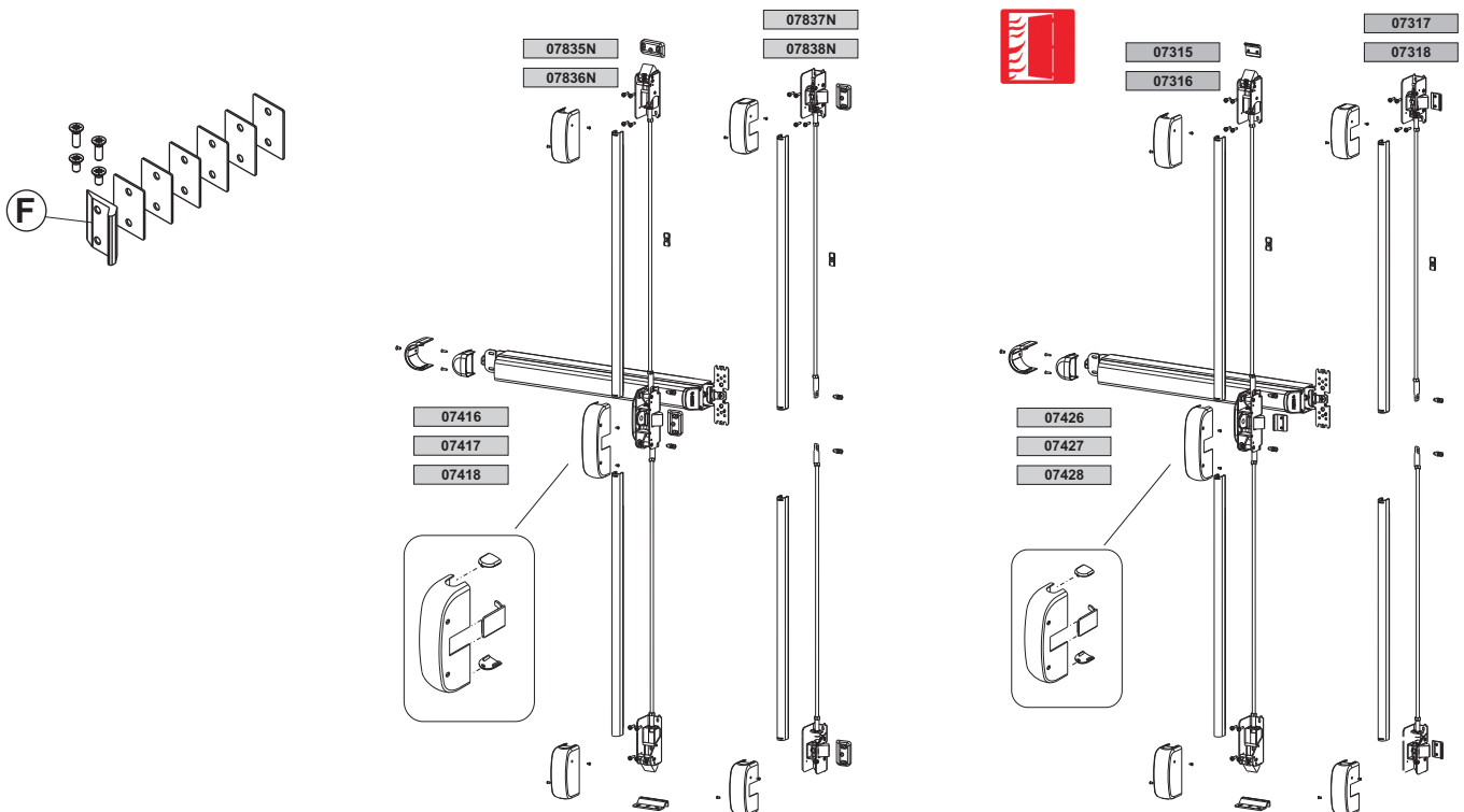
Standard version
