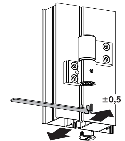
Compression adjustment
