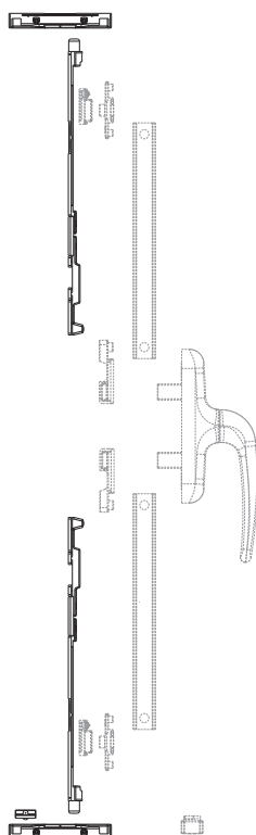
Passador monodirecional
