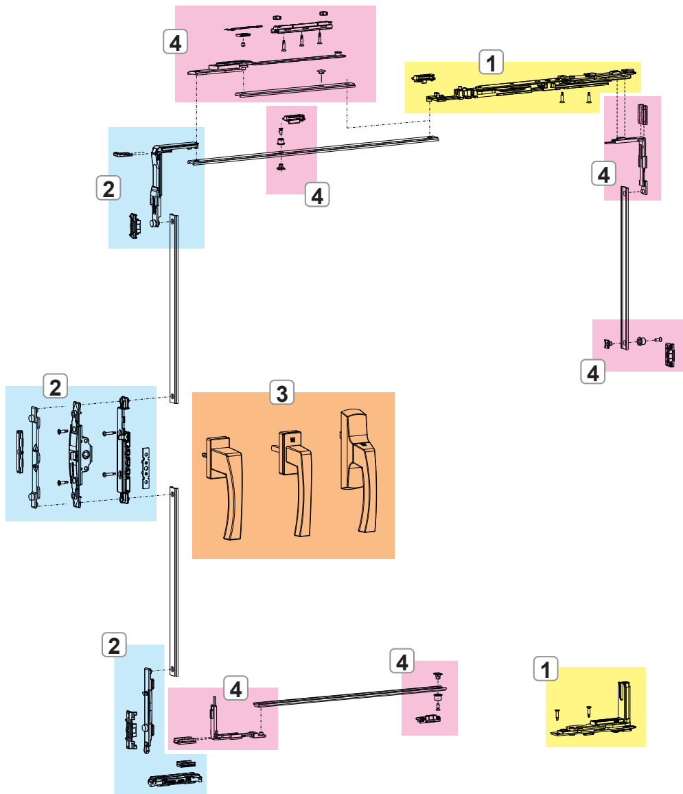
CHIC 3D 100 padrão
